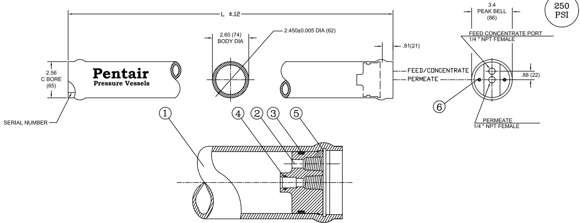
SECTION THROUGH END CLOSURE
